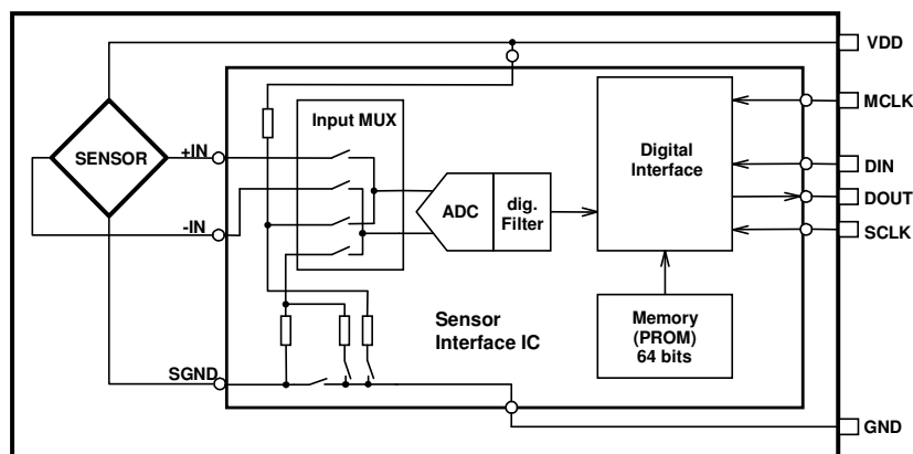
Fig.: 1 Block Diagram MS5536C
